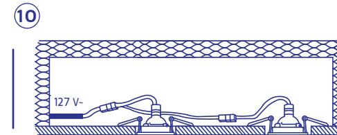
Diagram to install a 127 V~ lamp
